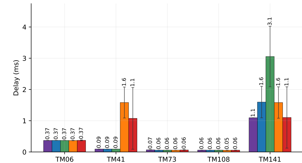
(c) Average Link Delay ↓
